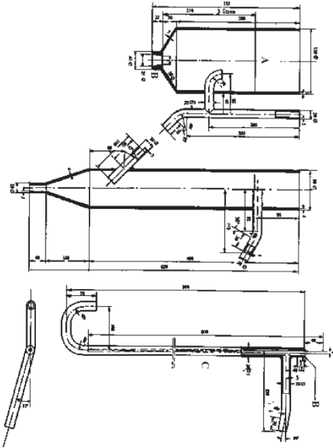
Figure 2 Activated sludge plant: detail (dimensions in millimetres)
