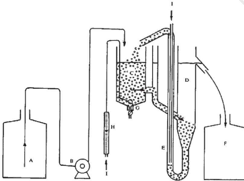
Figure 1 Activated sludge plant: overviews
