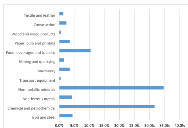
Graph A7.3: Gas consumption per industry, in thousands of terajoules – 2021
