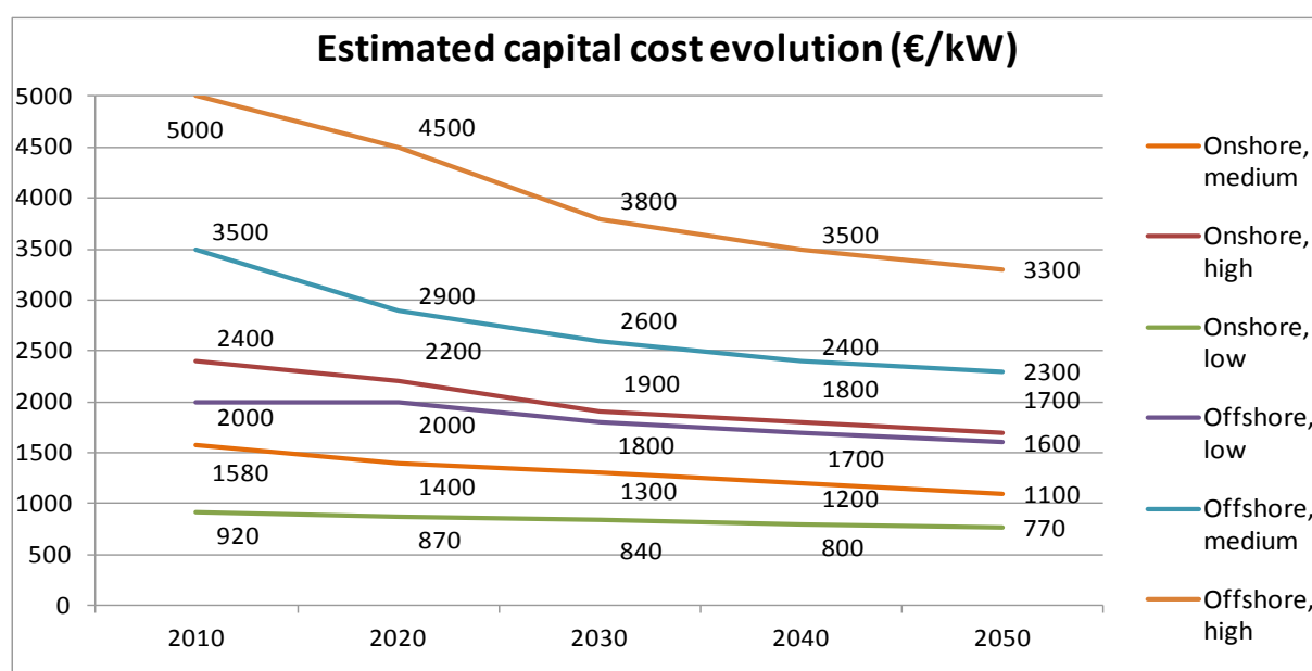
Figure 5.3: Expected evolution of capital cost for new wind power installations, for low, medium and high cost ranges. Source: JRC estimates.
