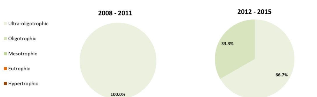
Figure 6. Saline water eutrophication classification during the previous and current reporting period ( coastal waters only, at three sites ).
