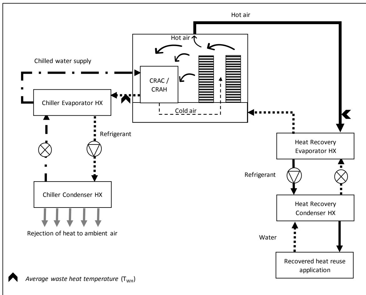
Figure 3: Measurement of waste heat temperature
