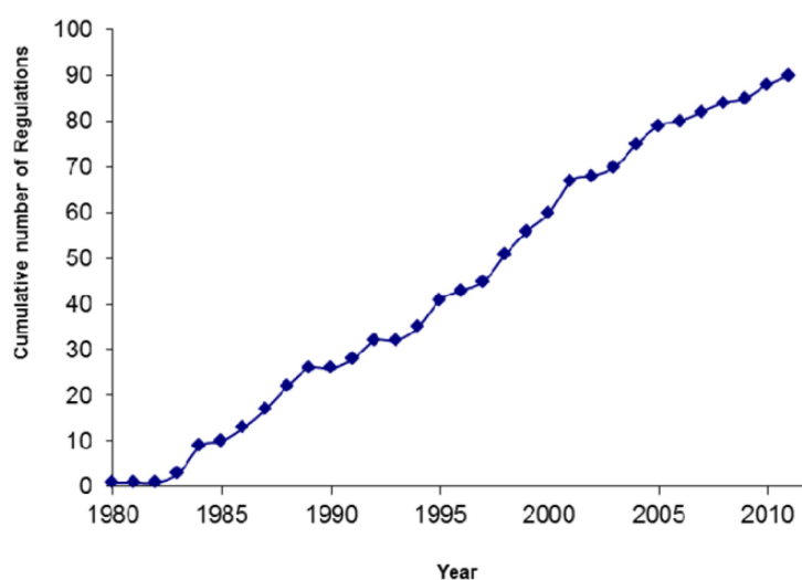
Figure 3.2.1: Cumulative number of technical measures regulations introduced since 1980 (Source: STECF 2012a page 18)
