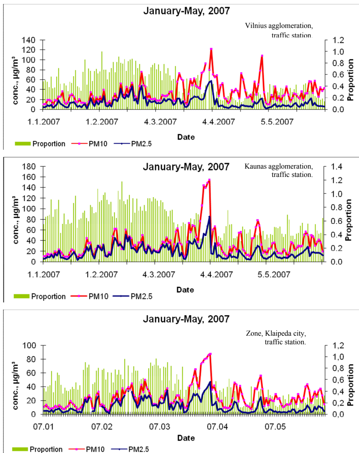
Figure 2: Concentrations of \text{PM}_{10} and \text{PM}_{2.5} , \text{PM}_{2.5}/\text{PM}_{10} ratios at kerb side locations in large cities in Lithuania, 2007 (source: Perkauskas, 2008)
