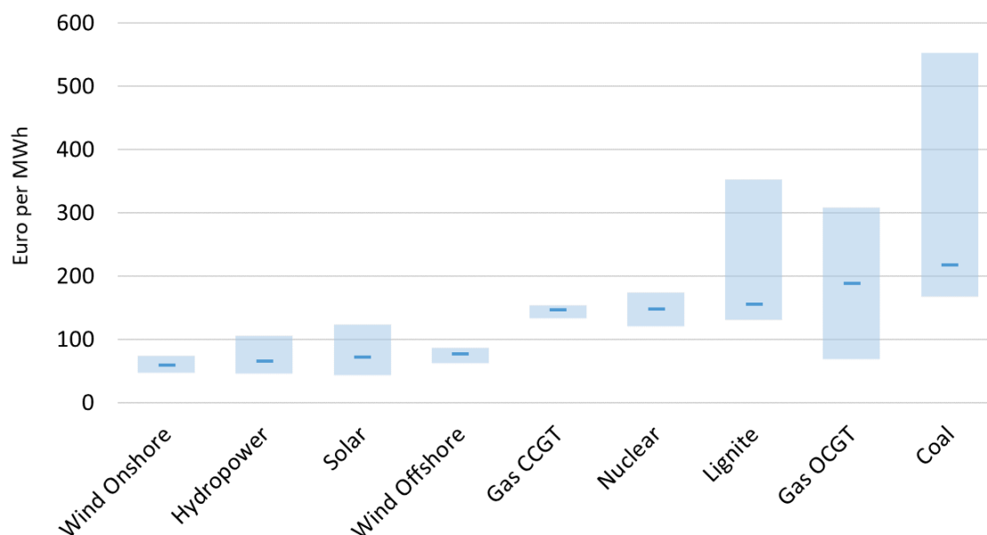
Figure 1: Snapshot of technology-fleet specific levelised costs of electricity (LCOE) for 2023. The solid blue lines denote the median and the light blue bars display a \pm 25\% range across the EU, highlighting differences among Member States.
