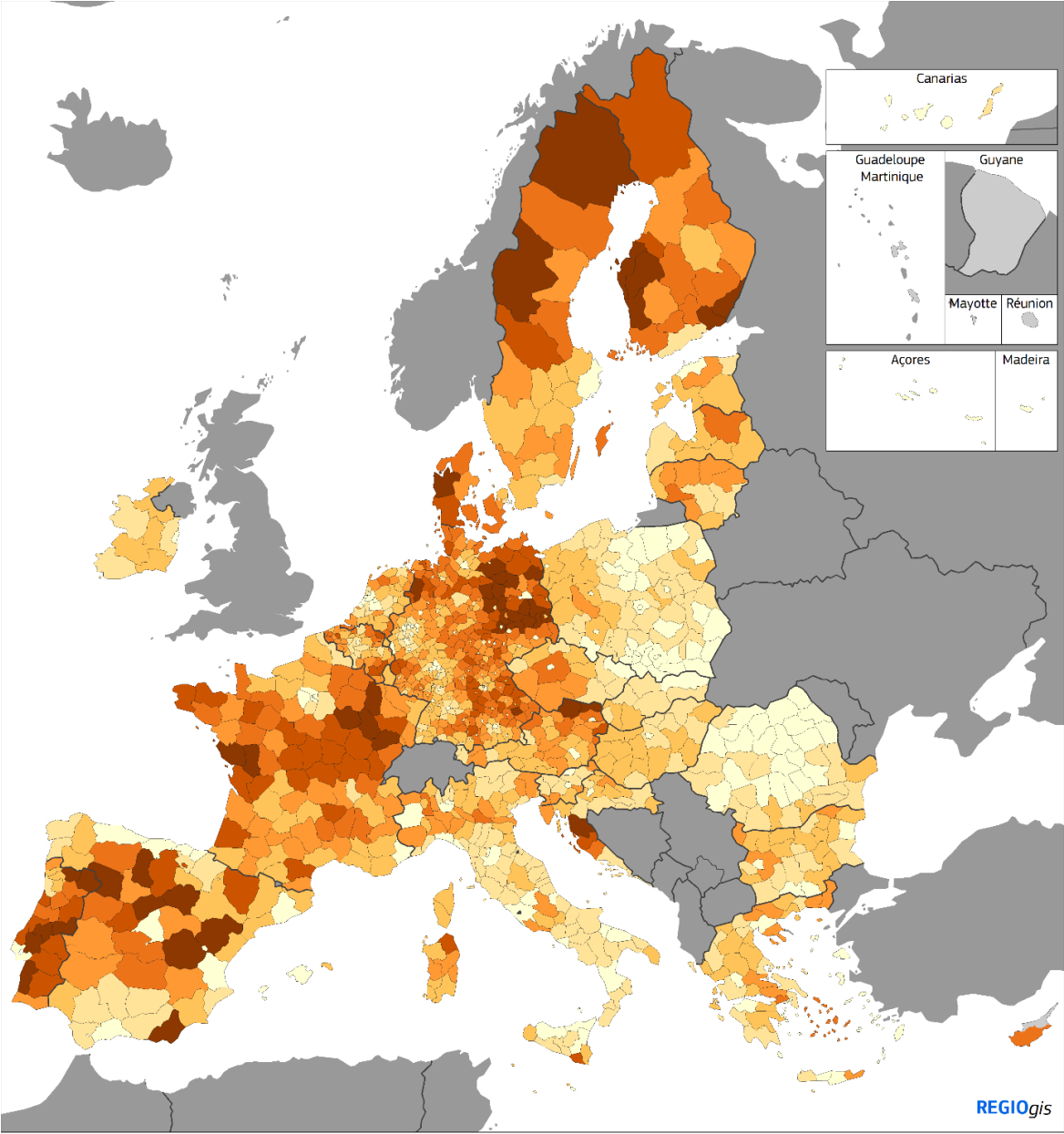
Imperviousness per inhabitant, 2018
