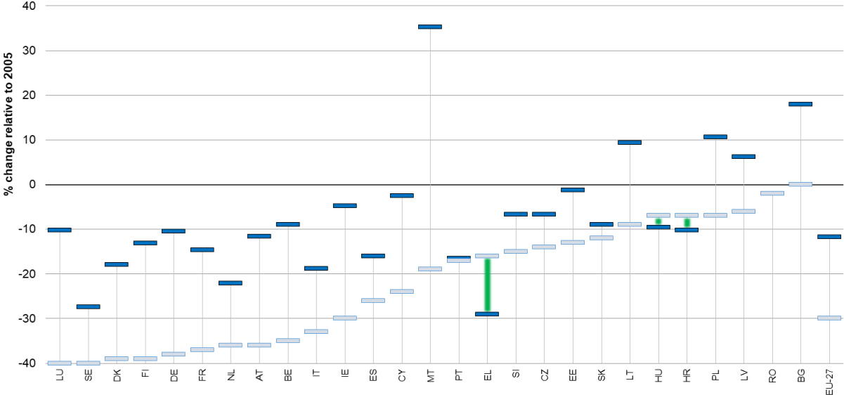
Figure 3-1 Change in greenhouse gas emissions outside the Emissions Trading Scheme, 2005-2018 and Europe 2030 targets
