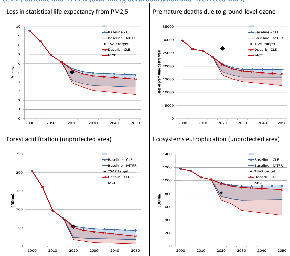
Figure A8.1: Impact reductions in the long term under different trajectories: current legislation (CLE) baseline and MTFR (blue lines), decarbonisation and MCE (red lines)
