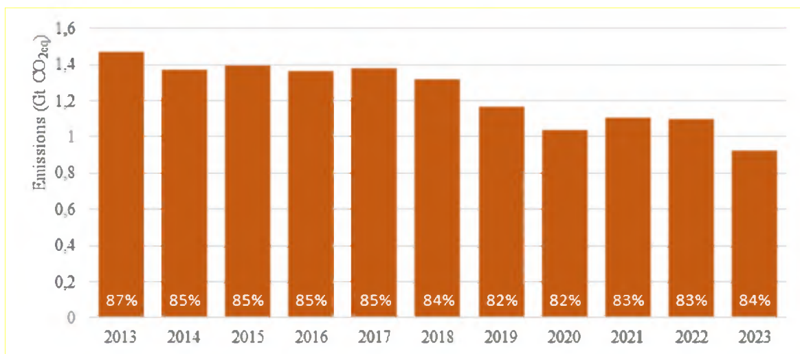
Figure 5. Trend in total emissions from fossil fuel combustion in installations covered by the EU ETS (2013-2023). Labels show the %-share of the installations' total emissions.
