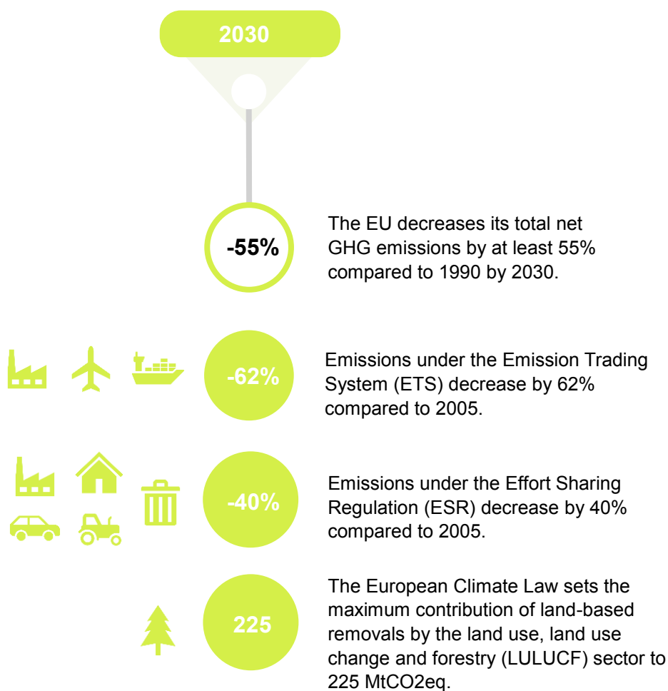
Figure 5: EU 2030 targets
