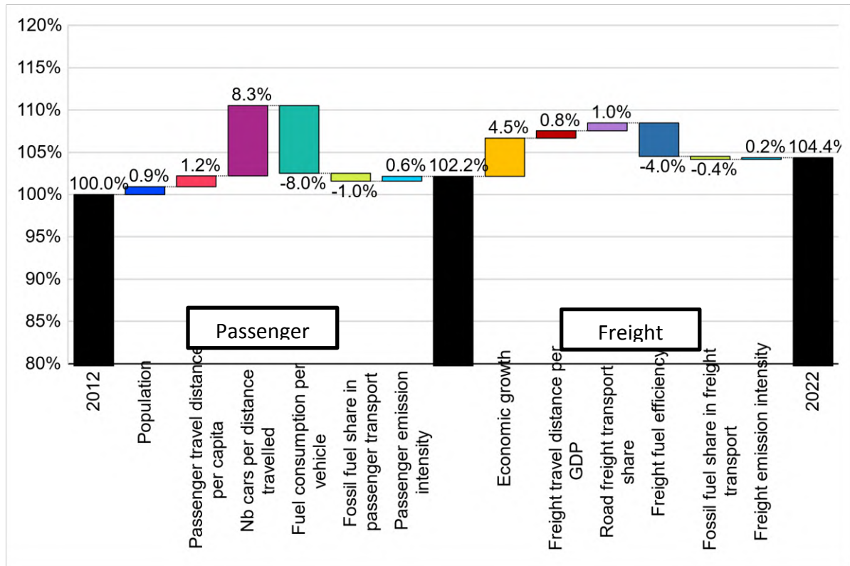
Figure 26: Decomposition of emissions in domestic road transport (2012-2022)
