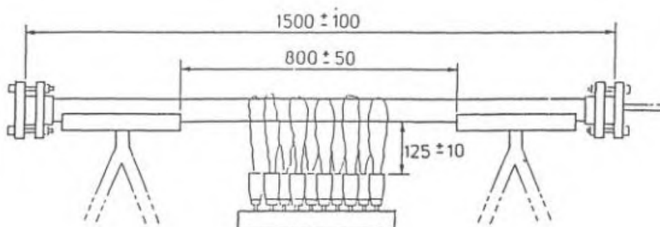
FIG. 2 FIRE ENDURANCE TEST, STAND WITH MOUNTED SAMPLE
