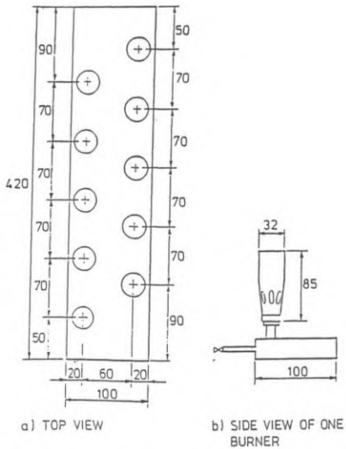
FIG. 1 FIRE ENDURANCE TEST BURNER ASSEMBLY
