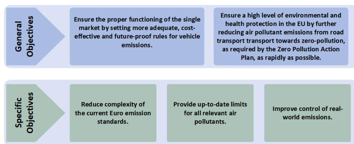
Figure 5 – Euro 7 objectives
