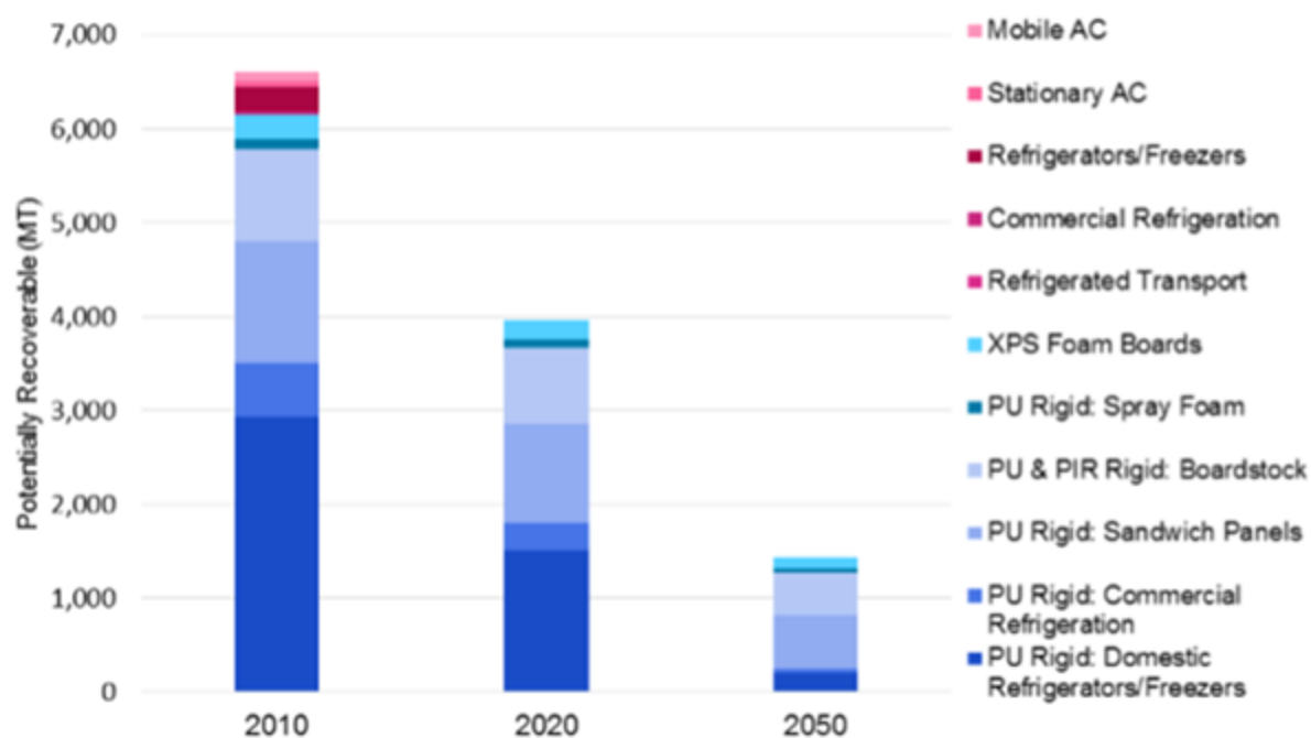
Figure 7 – Quantity of CFCs in metric tonnes that is potentially recoverable from retired EU equipment at its end-Of-Life (2010-2050)
