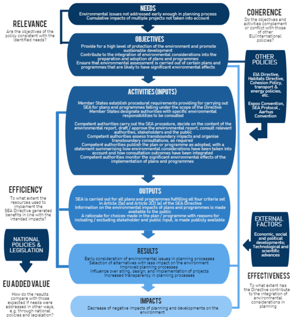
Figure 1: Intervention logic
