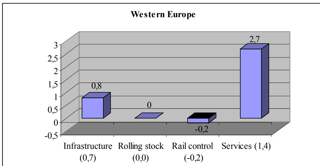
23b. Annual growth rates (in %) of the accessible and overall rail supply market segments 2005-2015 (figures in brackets show the total markets)
