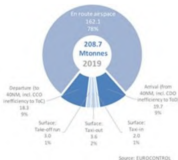
Figure 24 CO 2 emissions per flight phases
