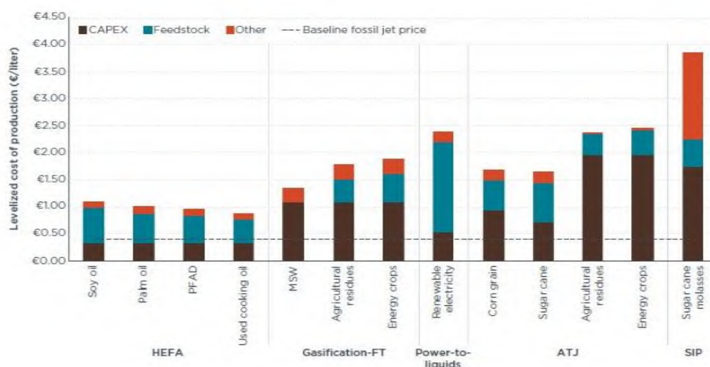
Figure 33 Current levelised costs of aviation fuels
