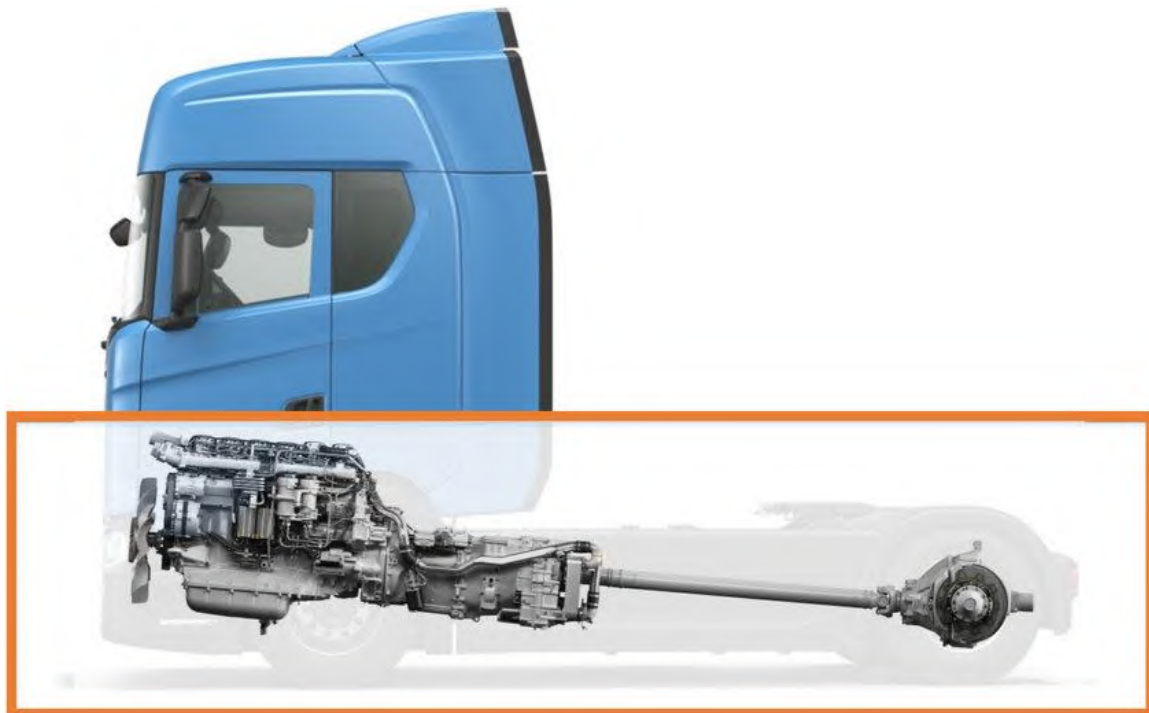
Figure 16: Truck powertrain
