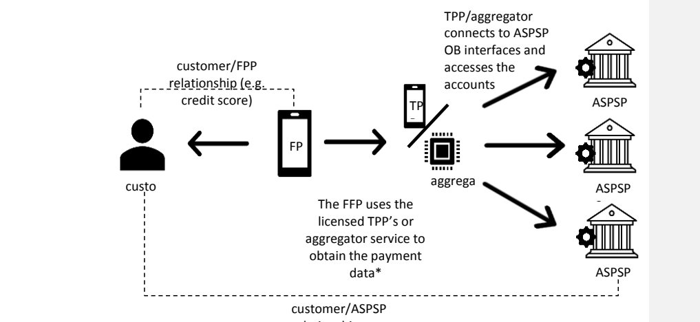
Figure 3 OB case with TPP/aggregator and unlicensed Fourth Party Provider
