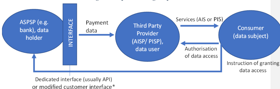
Figure 5: Open Banking simple case
