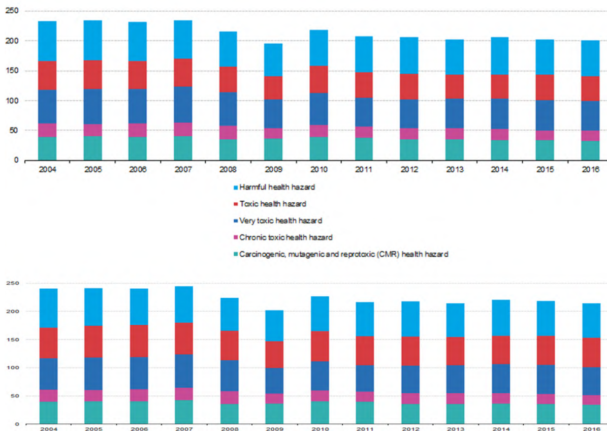
Figure 3 Production (1 st diagram) and consumption (2 nd diagram) of chemicals hazardous to health, EU-28, 2004-2016 (million tonnes). The different classes of chemicals are ranked according to their human health impact from the most harmful (bottom class) up to the least harmful (top class). Source: Eurostat (online data code: env_chmhaz)
