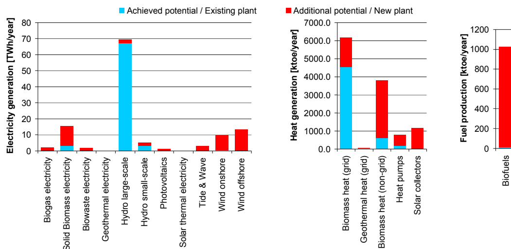
Figure 3: Mid-term potentials of RES electricity heat and transport in Sweden
