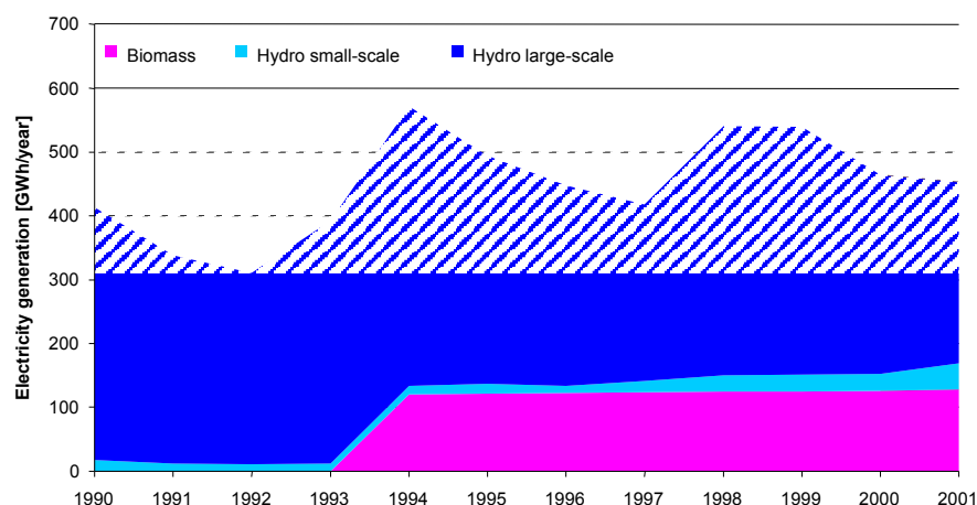
Figure 1: RES electricity production up until 2001 21 in Lithuania
