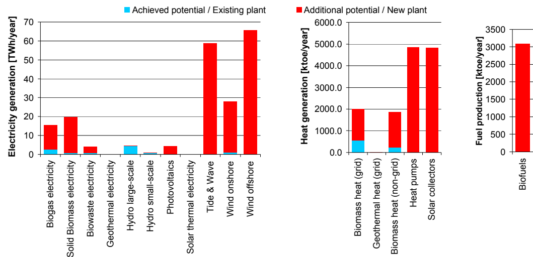
Figure 2: Mid-term potentials of RES electricity heat and transport in the UK
