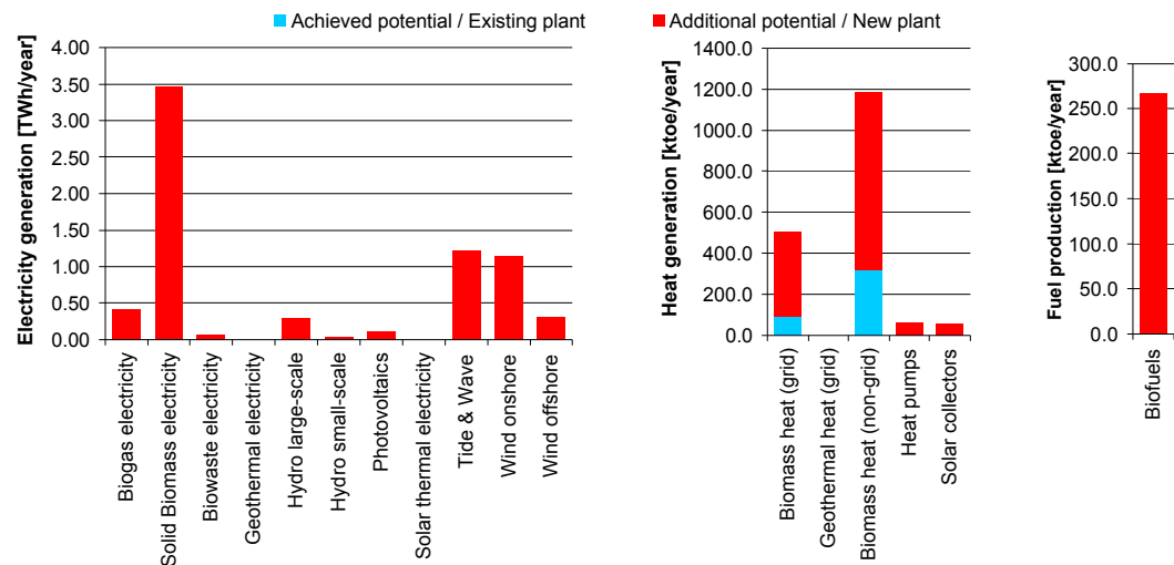
Figure 2: Mid-term potentials of RES electricity, heat and transport in Estonia
