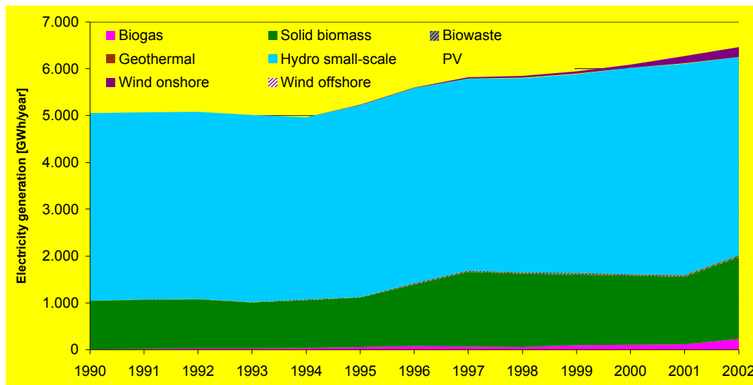
Figure 2: RES electricity production in Austria up until 2002 excluding large hydro
