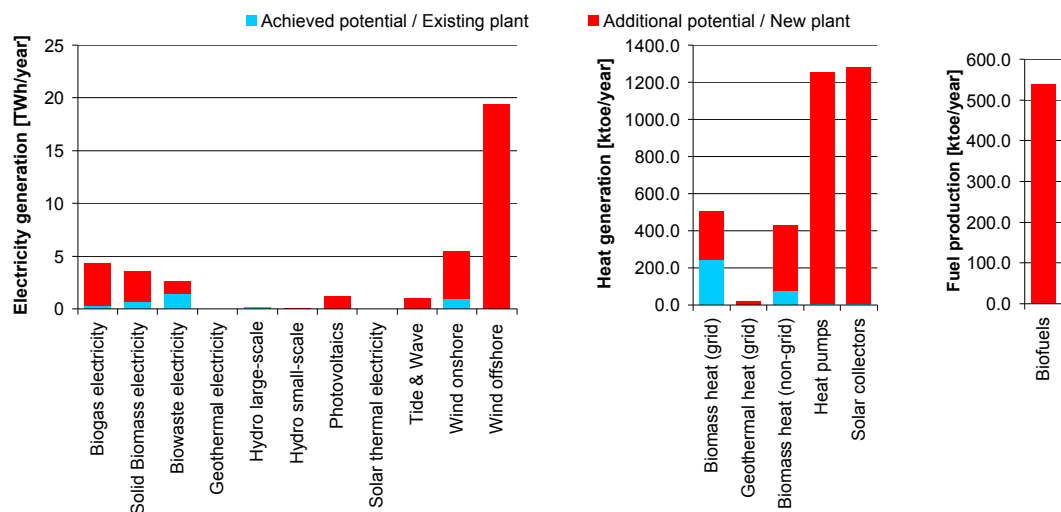
Figure 2: Mid-term potentials of RES electricity heat and transport in the Netherlands
