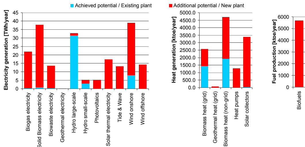
Figure 3: Mid-term potentials of RES electricity heat and transport in Spain
