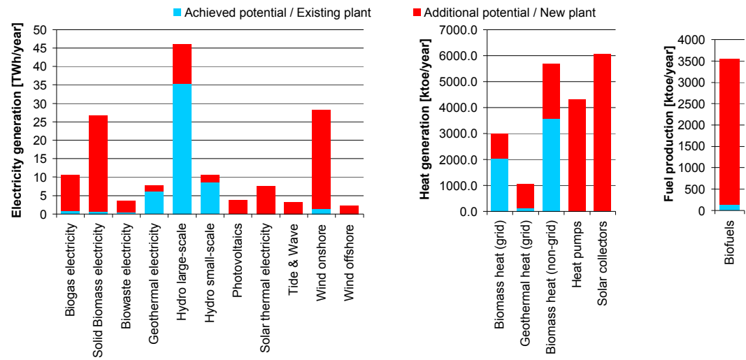
Figure 3: Mid-term potentials of RES electricity heat and transport in Italy
