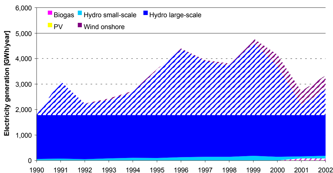
Figure 1: RES electricity production up until 2002 16 in Greece.
