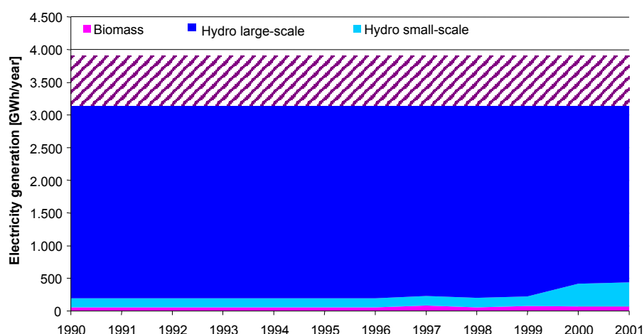
Figure 1: RES electricity production up until 2001 28 in Slovenia
