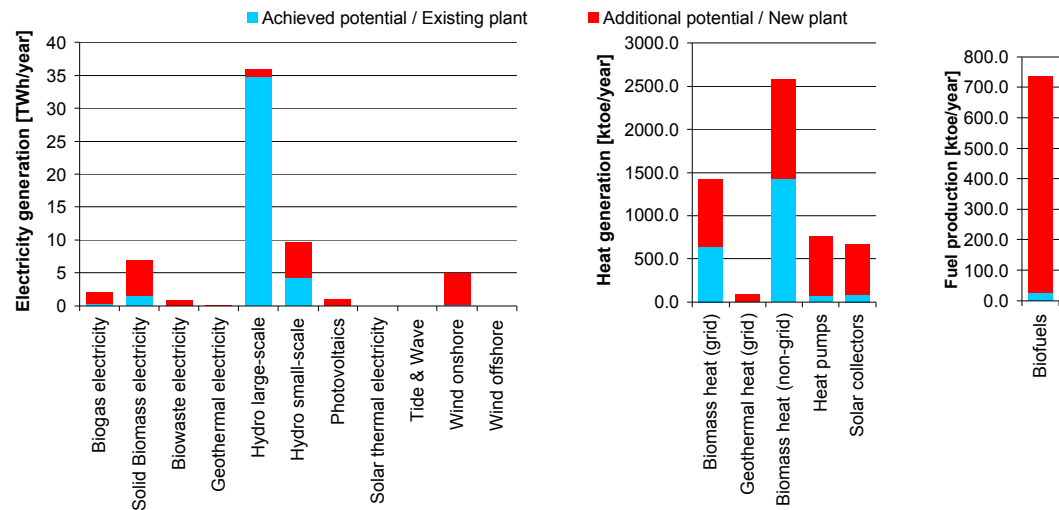
Figure 3: Mid-term potentials of RES electricity, heat and transport in Austria
