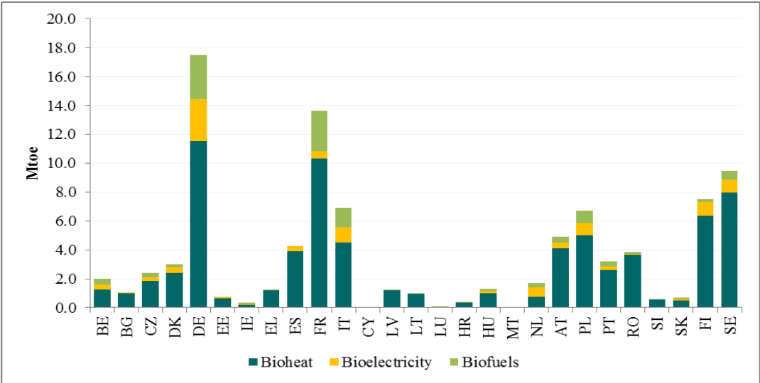
Figure 2: Final bioenergy demand by Member State (2012, Mtoe). Source: Member States Progress Reports on Renewable Energy
