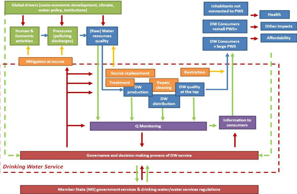
Figure 4: Scheme of the drinking water system
