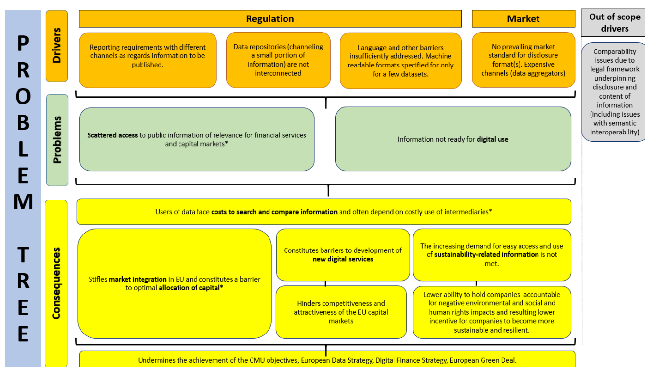
Figure 4: Problem Tree
