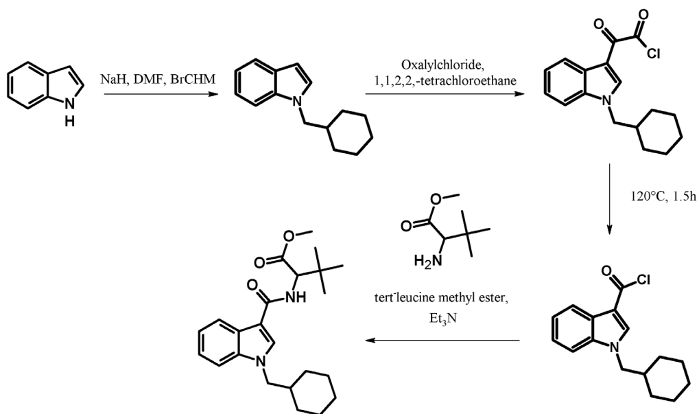
Figure 3: Possible synthetic route for MDMB-CHMICA starting from 1 H -indole – variant III
